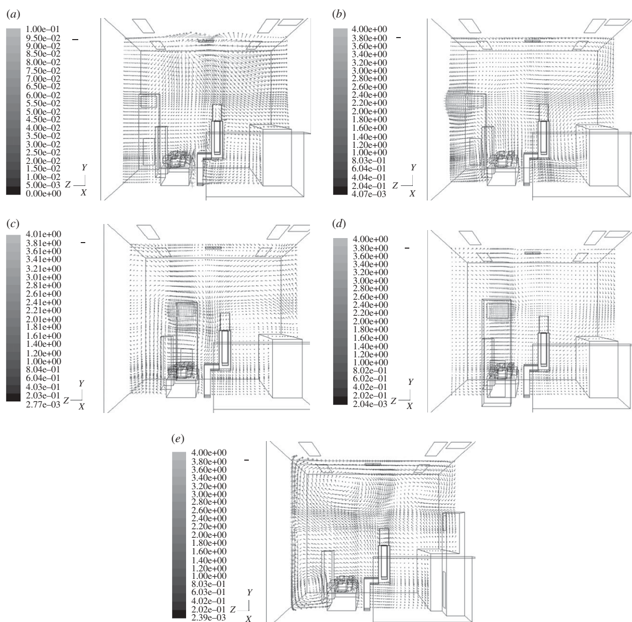
Figure 4. Velocity distribution for each case at X = 2.2 m. (a) Case 0, (b) case 1, (c) case 2, (d) case 3 and (e) case 4. Scale bar, (a) 0.1 \text{ m s}^{-1} ; (b–e) 0.5 \text{ m s}^{-1} .
